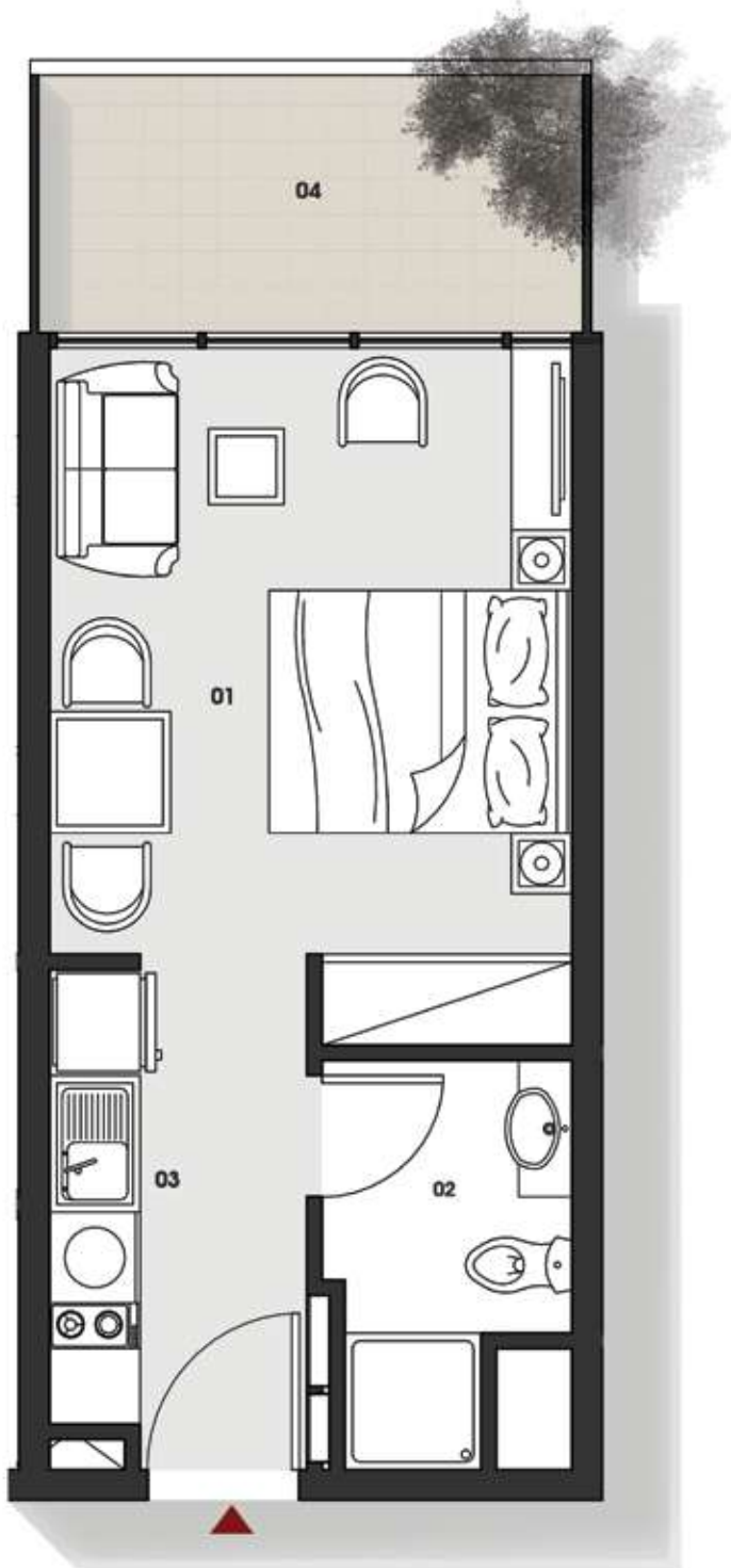
STUDIO PLAN 01 BEDROOM 3.4 x 4.0 m² 02 BATHROOM 1.6 x 2.7 m² 03 KITCHEN 3.0 x 1.7 m² 04 BALCONY VARIABLE
