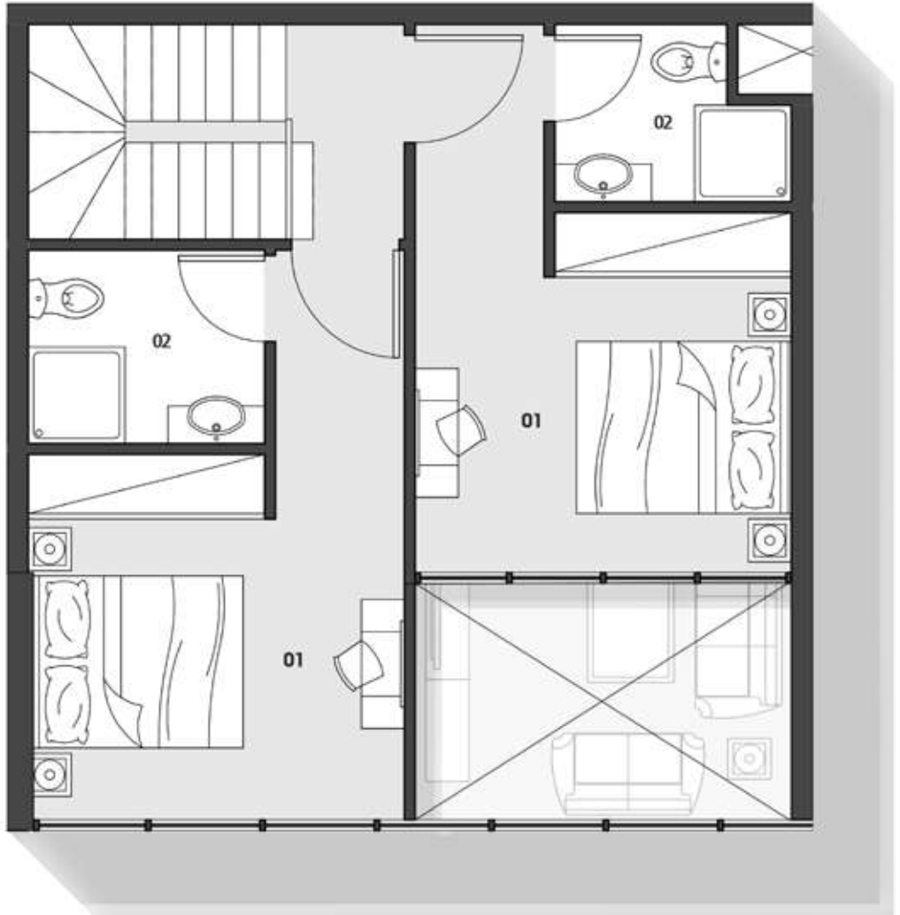
THREE BEDROOM LOFT PLAN UPPER LEVEL
